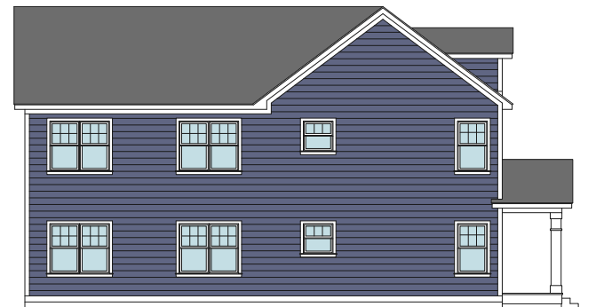
Side Elevation - Reverse Gabled Roof
